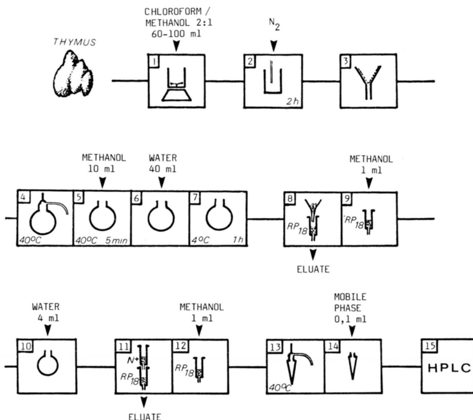
Fig. 1. [1] twentyfold volume of chloroform/methanol 2:1 to the tissue sample is added, [2] under N_2 atmosphere for 2 h, [3] filtration, [4] evaporation of the solvent, [5] addition of 10 ml methanol to the residue, [6] addition of 40 ml water, [7] 1 h cooling in a refrigerator, [8] filtering through glaswool and a Baker disposable extraction column RP_{18} , [9] elution with 1 ml methanol, [10] 4 ml water are added, [11] passing through a combination of a quaternary amine and a RP_{18} Baker disposable extraction column, [12] elution with 1 ml methanol, [13] evaporation of the methanol, [14] 0.1 ml from the mobile phase used in the HPLC separation system is added.
