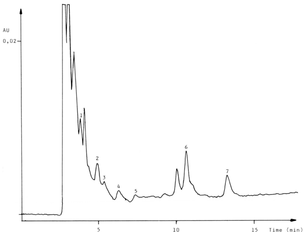
Fig. 2. Representative chromatogramme from an extract of a calf thymus, separated in system B. Peaks: 1 = progesterone, 2 = 20 \alpha -dihydroprogesterone, 3 = 17 \alpha -hydroxyprogesterone, 4 = 11 \beta -hydroxyprogesterone, 5 = 11-deoxycorticosterone, 6 = corticosterone, 7 = cortisol.
